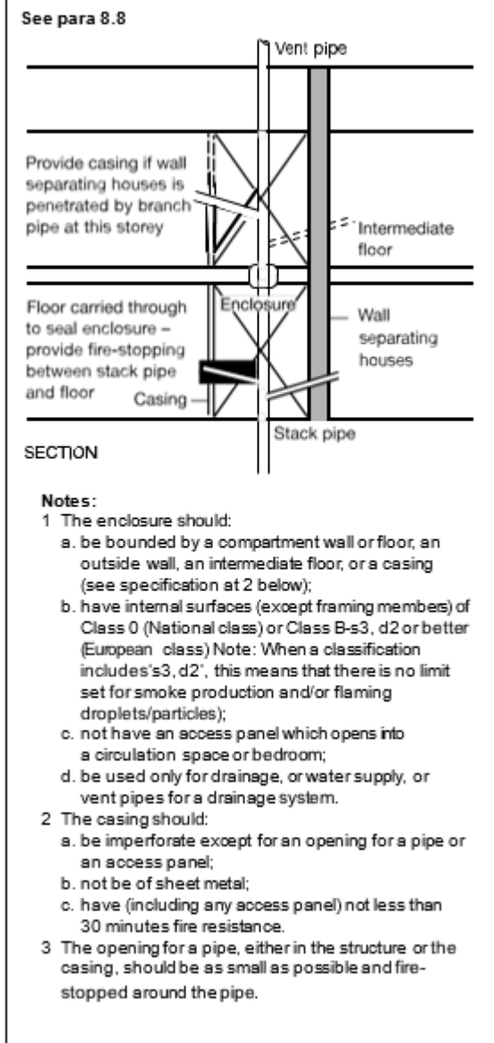
Diagram 15 Enclosure for drainage or water supply pipes
